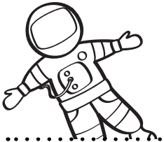
astronaut
