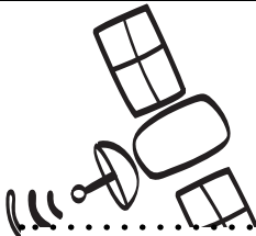
satellite
