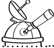
observatory
