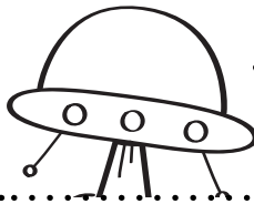
spaceship
