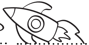
rocket
