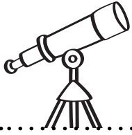
telescope
