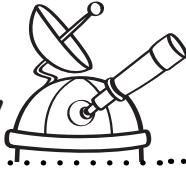
observatory
