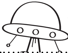
spaceship
