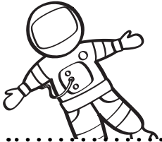
astronaut
