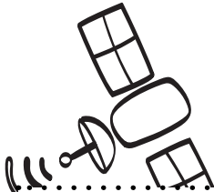
satellite
