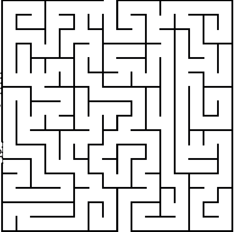
astronaut
